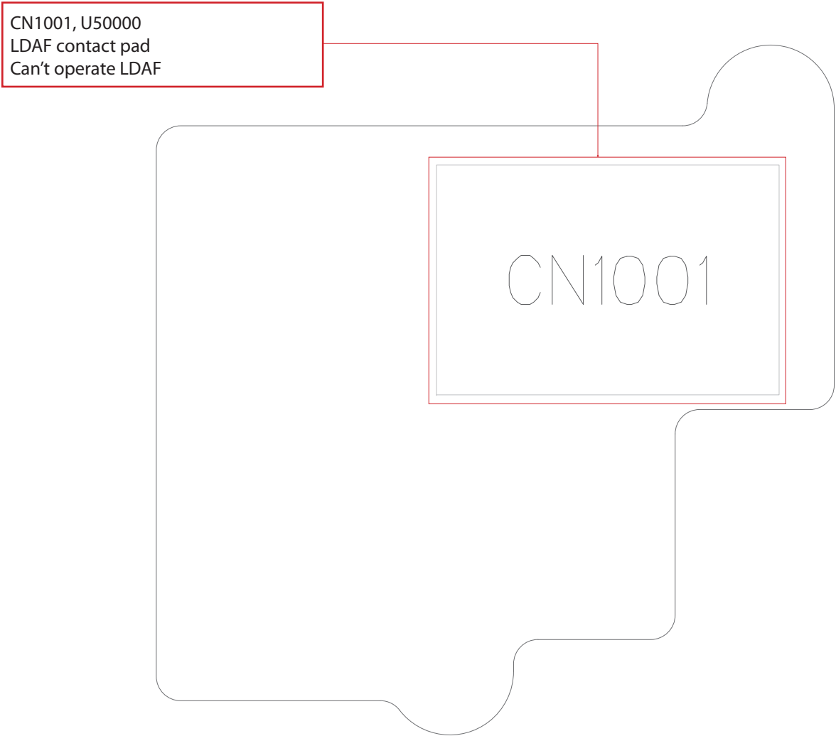
LDAF FPCB_TOP
