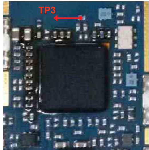
GPS RF Path & Test Point (Top)
