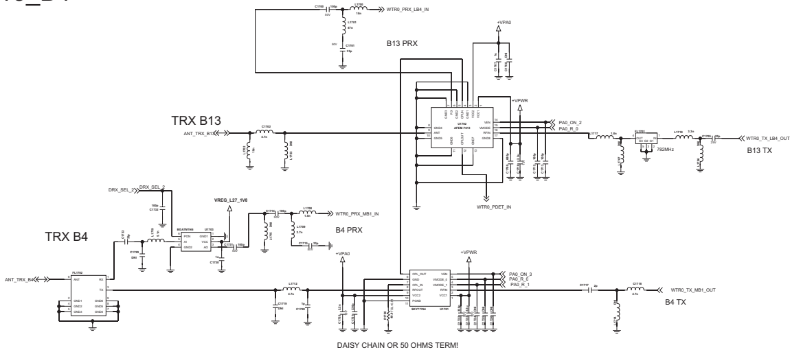
< 1-3-6-3_TRX_B13_B4 >
